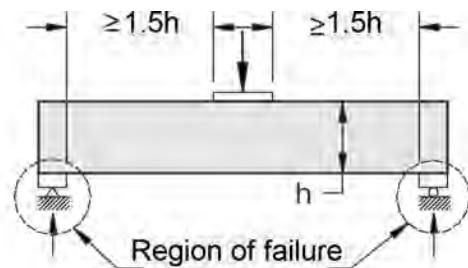
End One Flange Loading (EOF)
