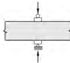
Interior Two Flange Loading (ITF)
