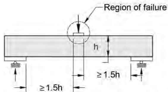
Interior One Flange Loading (IOF)
