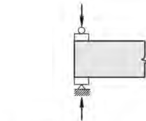
End Two Flange Loading (ETF)
