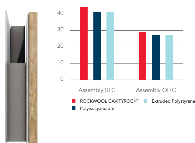
Test Wall: (Inside to Outside) 1/2" Gypsum, 6" Steel stud, Gypsum board, Air/Vapor retarder, ROCKWOOL CAVITYROCK® insulation, Airspace, 3/8" Cement board cladding.
