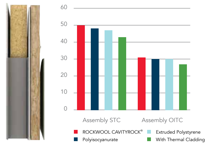
Test Wall: (Inside to Outside) 1/2" Gypsum, 6" Steel stud, ROCKWOOL COMFORTBATT® insulation, 5/8" Gypsum board, Air/Vapor retarder, ROCKWOOL CAVITYROCK® insulation, 3/8" Cement board cladding.
