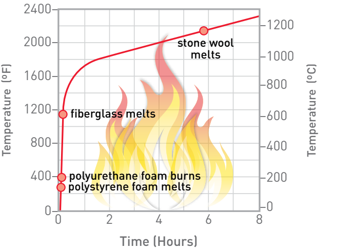
Temperature Development in a Standard Fire (ASTM E119)
